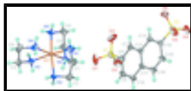
Fig. 1. A displacement ellipsoid plot of [\text{Ni}(\text{en})_3] ( \text{C}_{10}\text{H}_6\text{O}_6\text{S}_2 ) at the 50% probability level; hydrogen atoms are drawn as spheres of arbitrary radius; the disorder in the –SO 3 is not shown.
